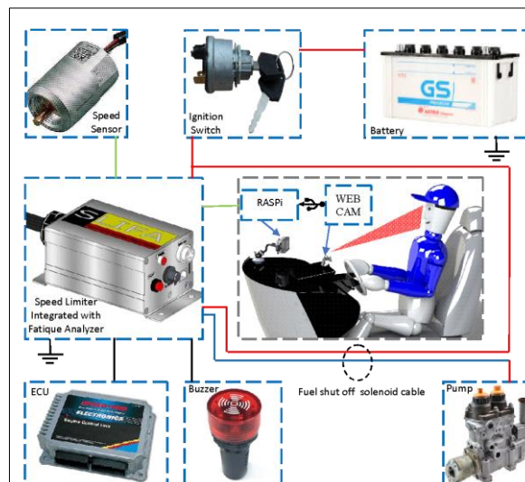
Figure 2. SLIFA Installation Diagram + Sleep Detector
