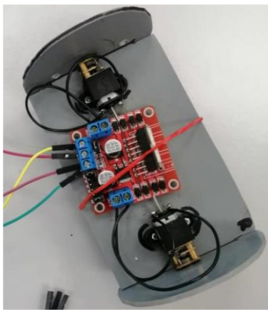
Figure 5. Incomplete MedSAT chassis
